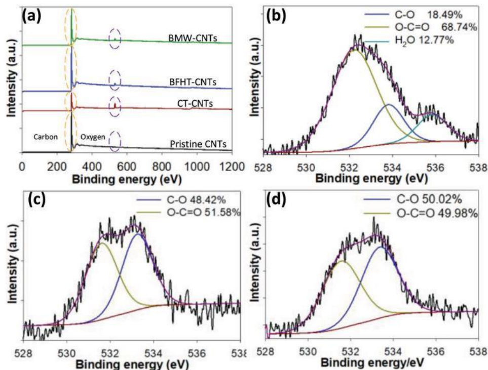
Figure 2. a) XPS spectra of the pristine CNTs, CT-CNTs, BFHT-CNTs, and BMW-CNTs. Deconvolutions of the XPS O1s of b) CT-CNTs, c) BMW-CNTs, and d) BFHT-CNTs.
