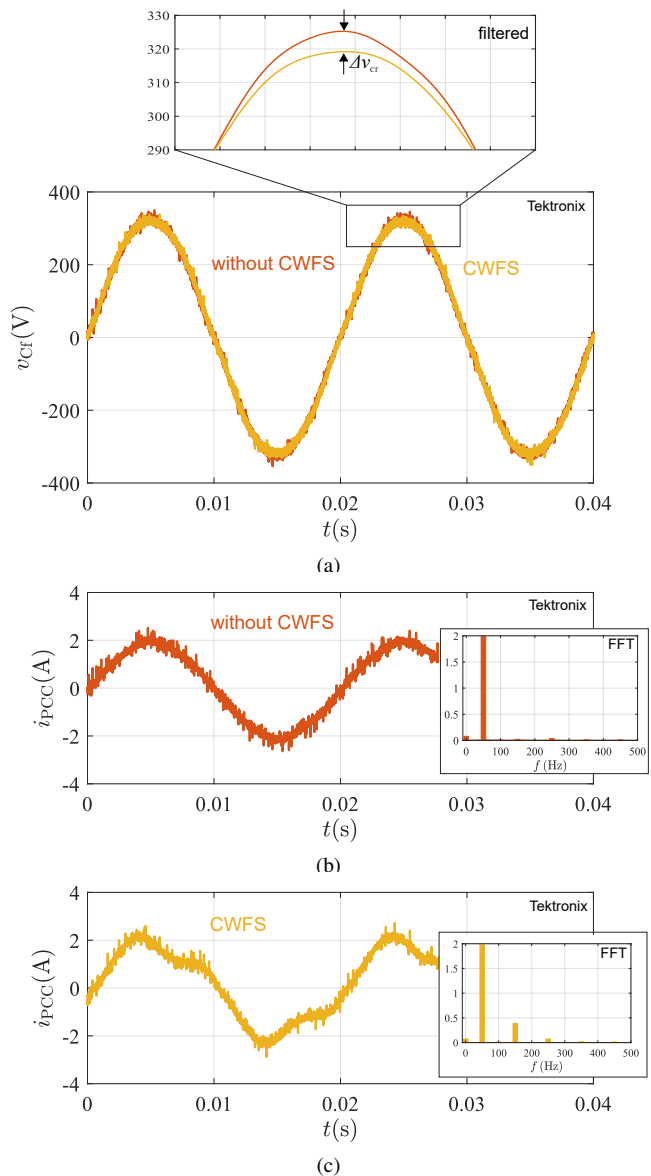
Fig. 16. Grid operation without and with CWFS ( \hat{I}_{1,inv}^* = 2 A): (a) Comparison of grid filter capacitor voltage waveforms, (b) PCC current without CWFS, (c) PCC current with CWFS.
