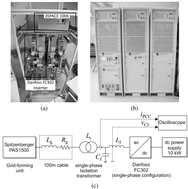
Fig. 15. Experimental setup: (a) Danfoss inverter system (FC302) in single-phase configuration, (b) Spitzberger PAS1500, (c) setup overview.
